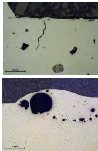
Arc welding (GTAW) evaluations
