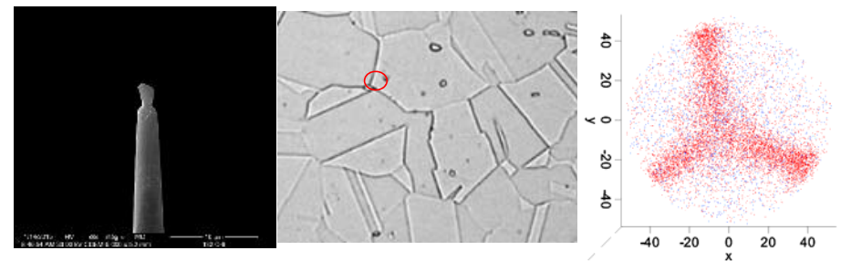
Boron distribution evaluation (atom probe)
