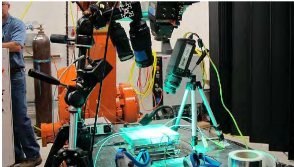
Digital Image Correlation (DIC) – Experimental Setup
