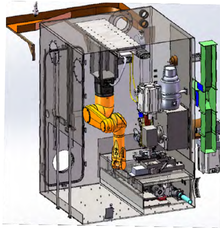
Welding Hot Cell Design with welding processes
