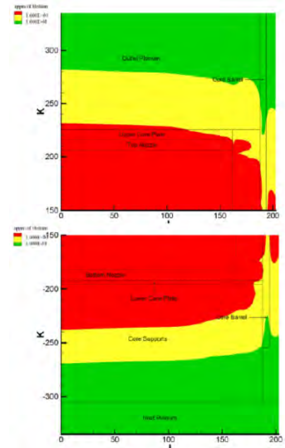
Typical He generation plot (10 wppm initial boron)
