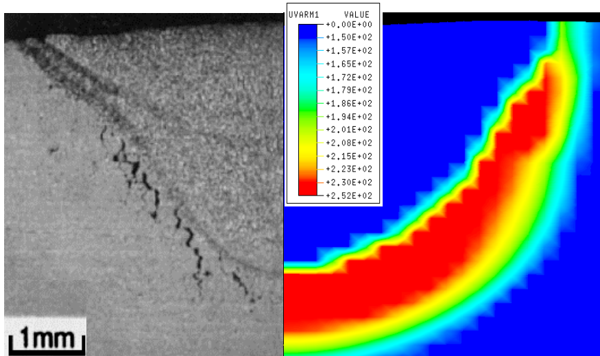
High Tensile Residual Stresses Modeled
