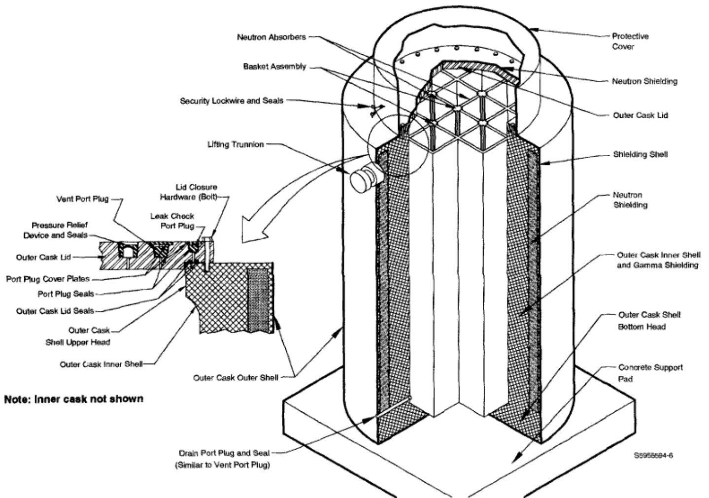
Figure 8. Vertical Metal-Shielded Dry Cask System Used with permission of Holtec International
