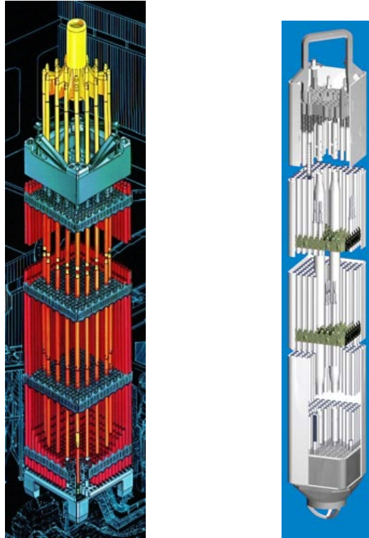
Figure 1. Typical Pressurized-Water Reactor (left) and Boiling-Water Reactor Fuel Assemblies
