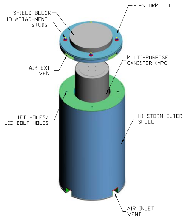
Figure 7. Typical Canister-Based Storage System
