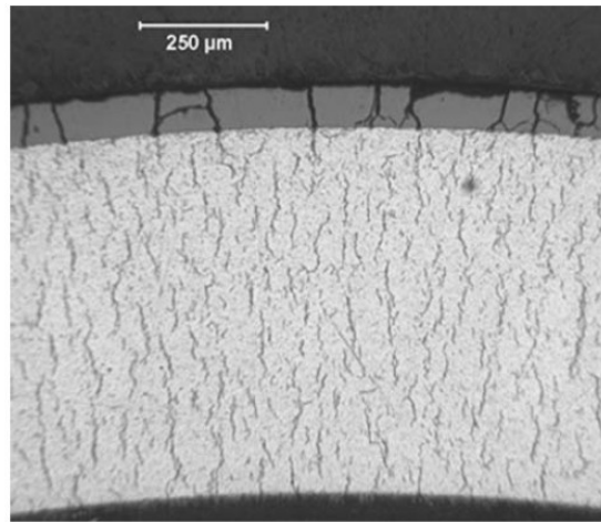
Figure 35. Large Radial Hydrides in High-Burnup Fuel-Rod Cladding After Cooling 137
