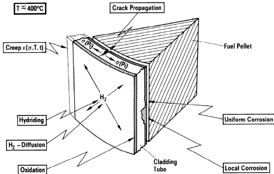
Figure 33. Mechanisms Affecting Used-Fuel Cladding Performance During Dry Storage 126
