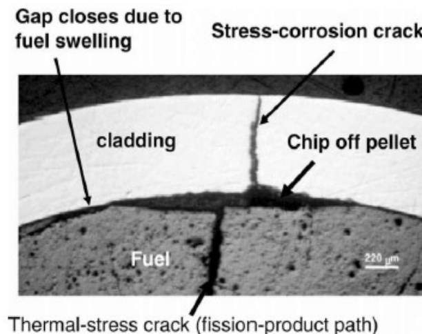
Figure 24. Stress-Corrosion Cracking of Cladding 46
