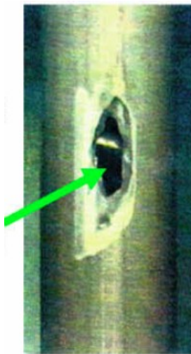
Figure 22. Fretting Wear Leading to Cladding Breach at Grid Spacer 62
