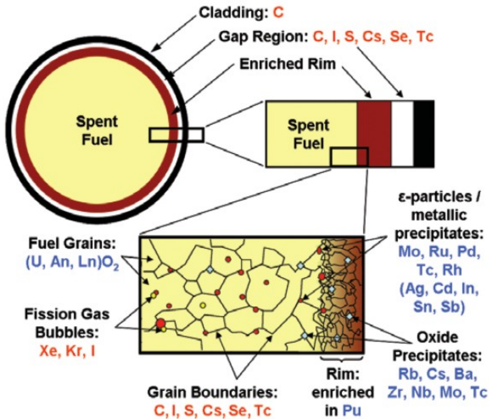
Figure 15. Schematic Illustration of the Microstructure of Used Fuel-Pellet and the Distribution of Actinides and Fission Products Following Burnup in a Reactor 5
