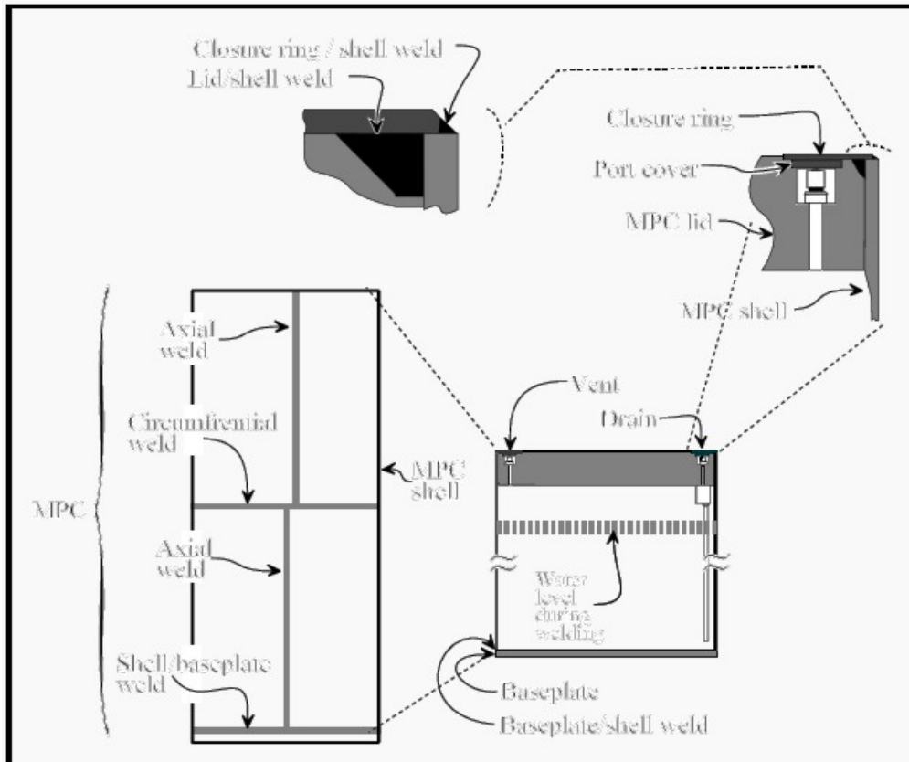
Figure 25. Drawing of Holtec HI-STORM 100 MPC Construction with Weld Locations (best available figure) 84
