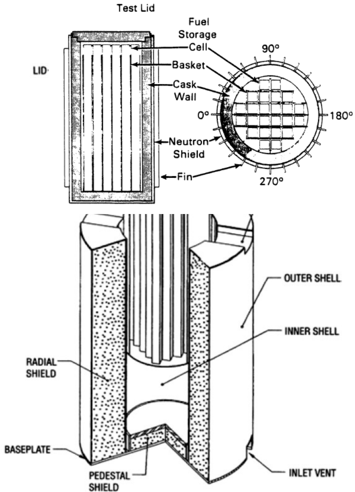
Figure 9. Vertical Welded-Canister Concrete-Shielded Dry-Storage System
