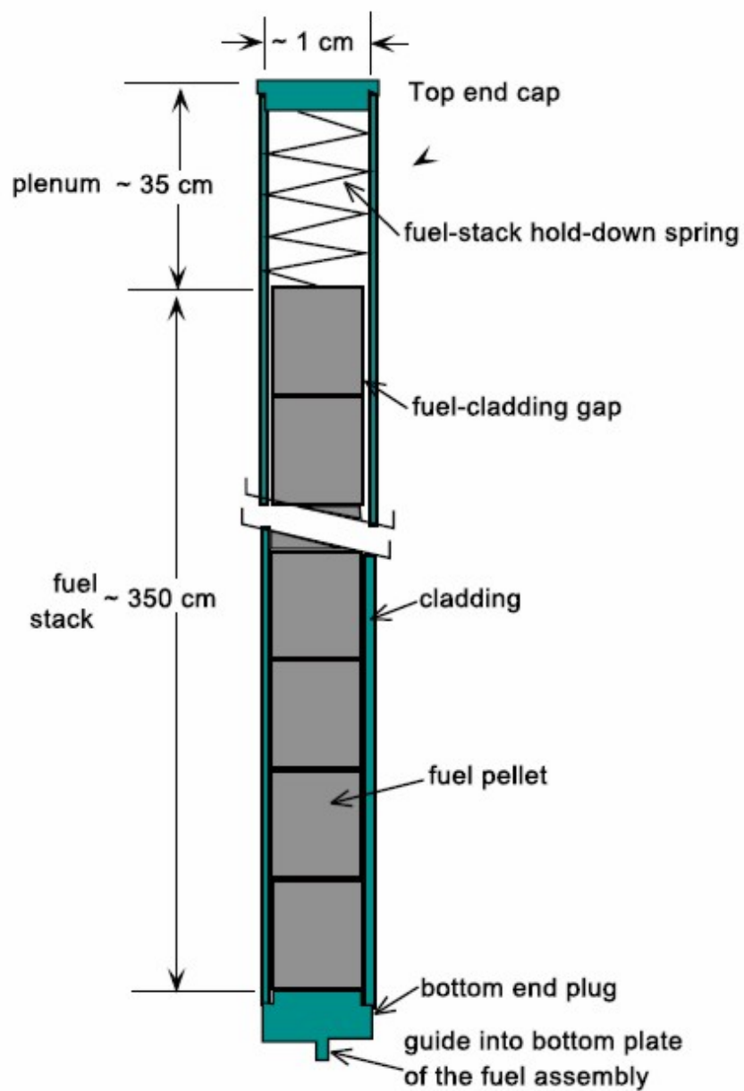
Figure 17. A Generic LWR Fuel Rod 51
