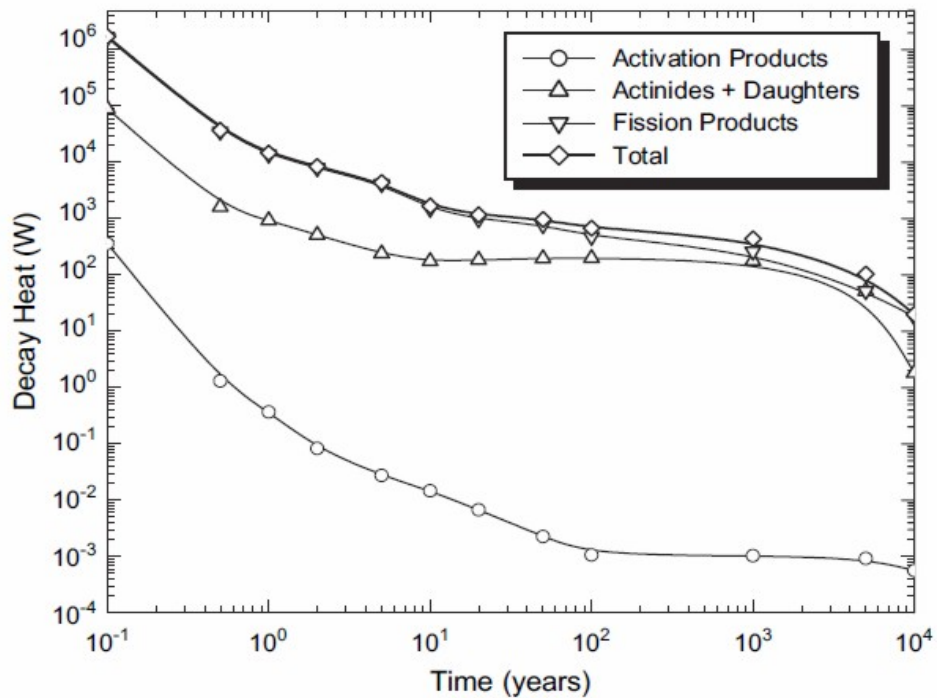
Figure 30. The Variation of Decay Heat for 10,000 Years for a Typical 30 GWd/MTU Burnup PWR CSNF 84
