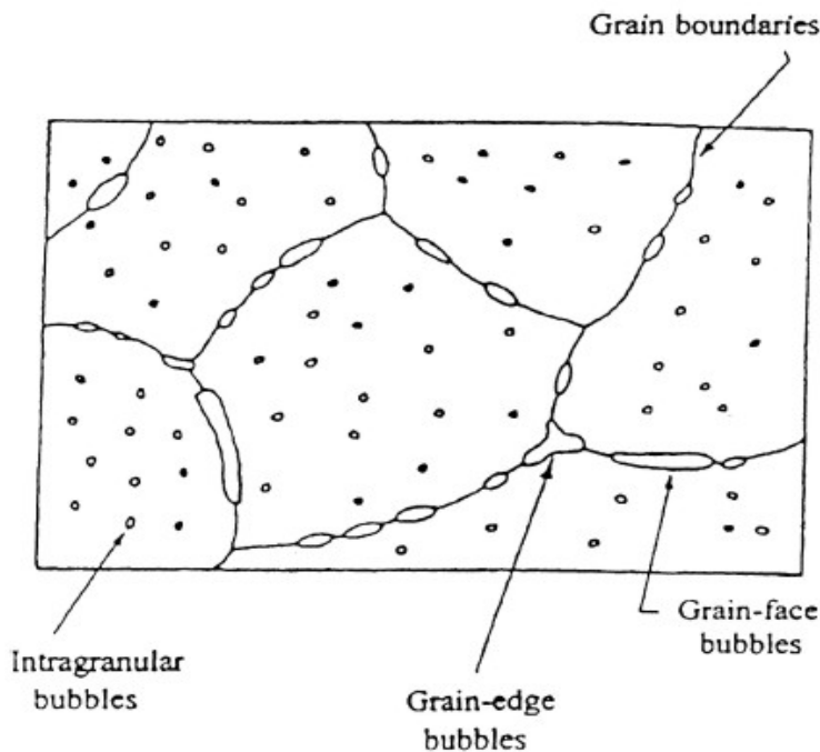
Figure 32. Schematic Cross Section of Granular Fuel-Pellet with Gas Products 112
