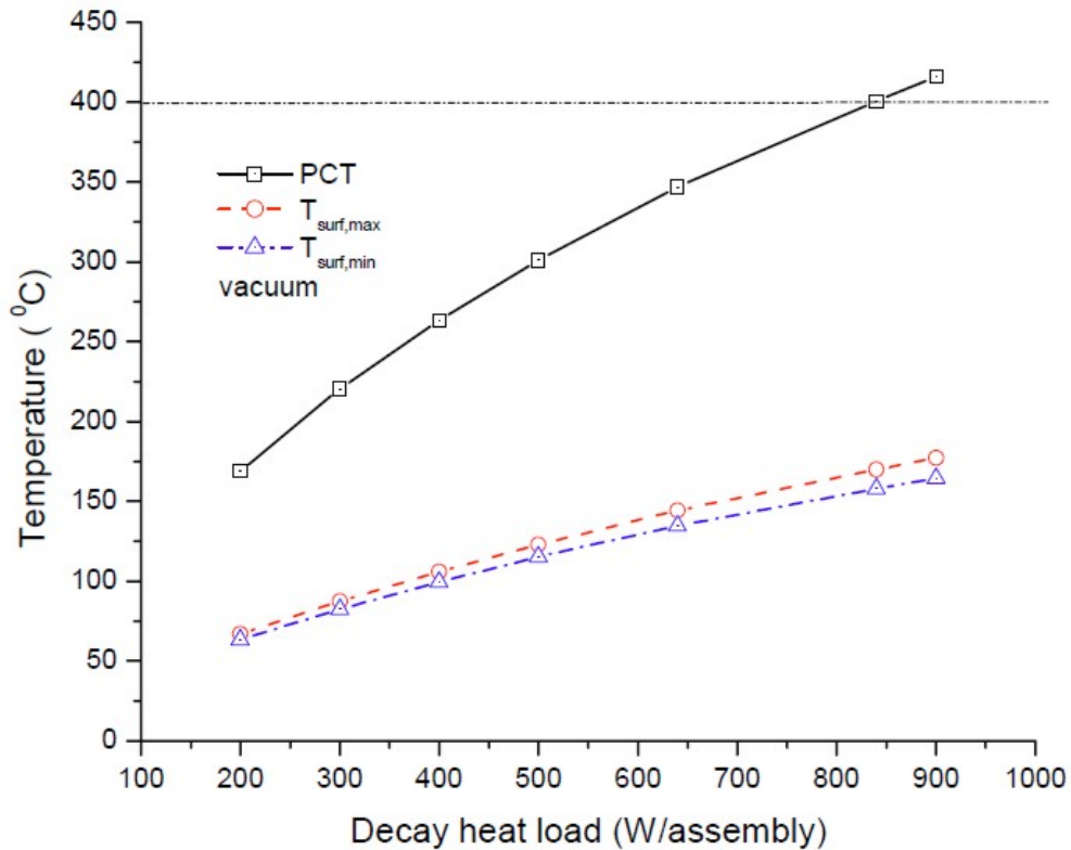
Figure 23. Calculated Peak Cladding Temperature (PCT) and Canister Surface Temperatures as a Function of Assembly Decay Head Load for an Evacuated Canister Containing 21 PWR (15 x 15) Assemblies 83
