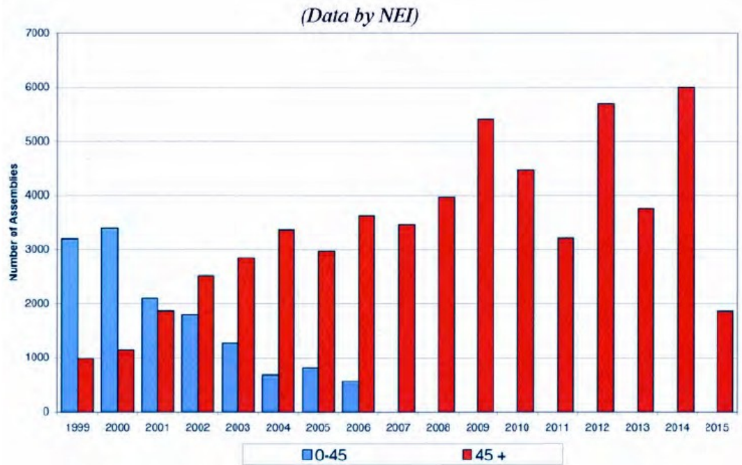
Figure 26. Projected BWR Burnup Distribution Through 2015 89 (Note: graph units are GWd/MTU)
