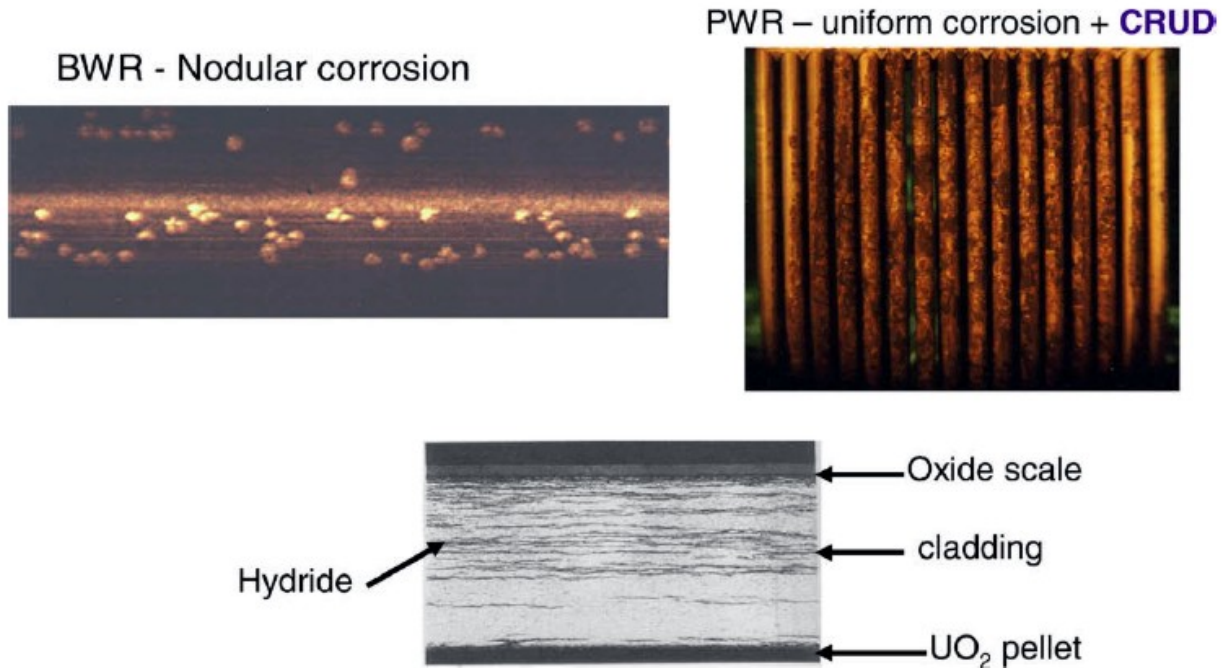
Figure 19. Corrosion of Zirconium-Alloy LWR Cladding 62
