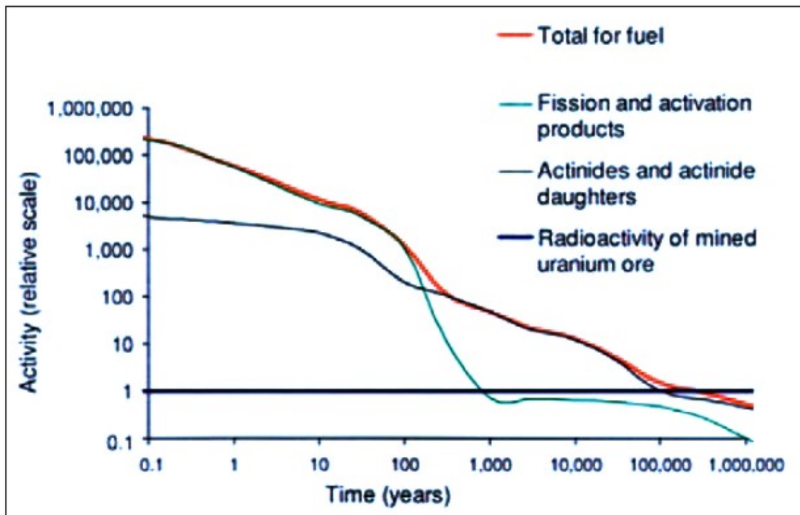
Figure 28. Relative Radioactivity of Used Nuclear Fuel with a Burnup of 38 GWd/MTU 5
