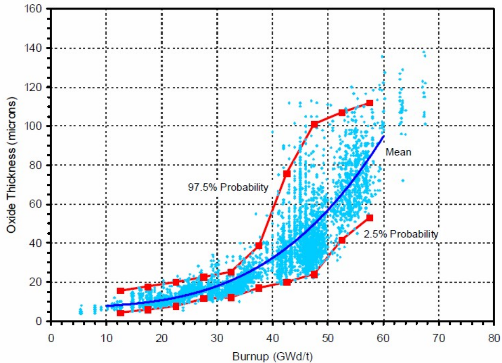
Figure 20. Cladding Outer Surface Oxide Layer Thickness Versus Rod Average Burnup 63
