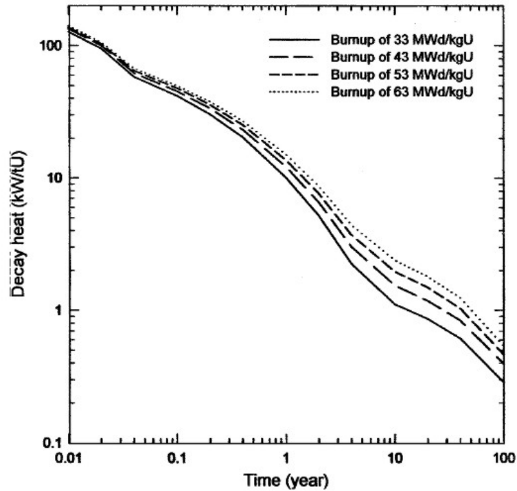
Figure 29. Decay Heat as a Function of Time from 0.01 Years (about 4 Days) to 100 Years for Used-Fuel Burnups of 33, 43, 53, and 63 GWd/MTU Where 33 Was Typical for the 1970s and 50+ for Current Burnups 91
