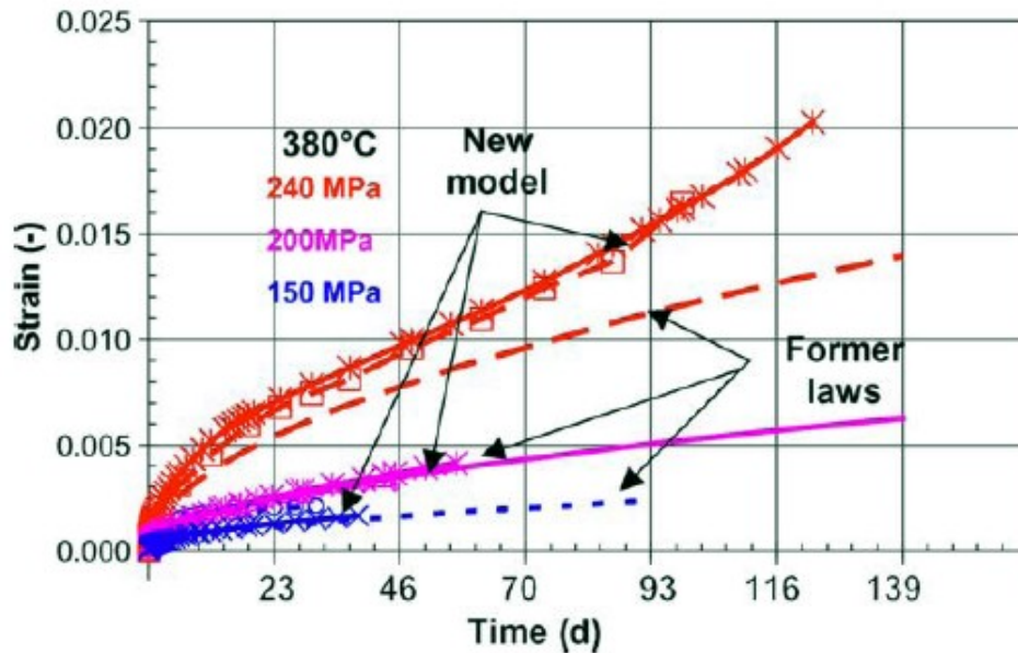
Figure 34. Comparison of Cladding Creep Models at Different Tube Hoop Stresses 109
