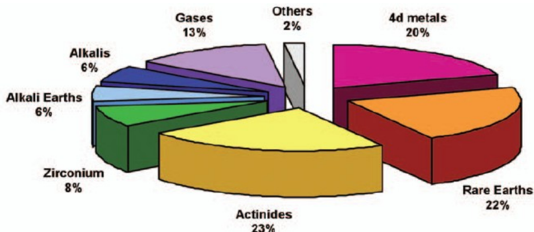
Figure 16. Pie Diagram Showing the Relative Proportions of the Major Fission Product and Transuranium Elements Found in Used Fuel-Pellets at Moderate Burnup 5
