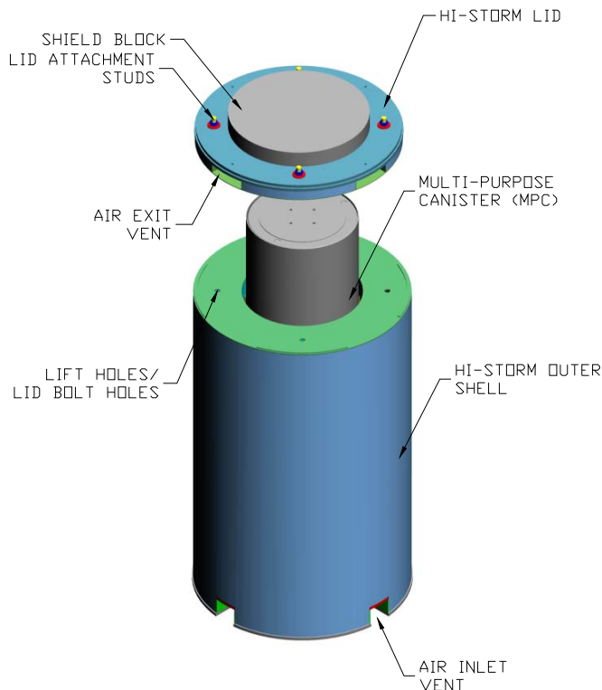
Figure 4. Typical Vertical Dry Cask-Storage System Graphic Courtesy of Holtec International, Inc.
