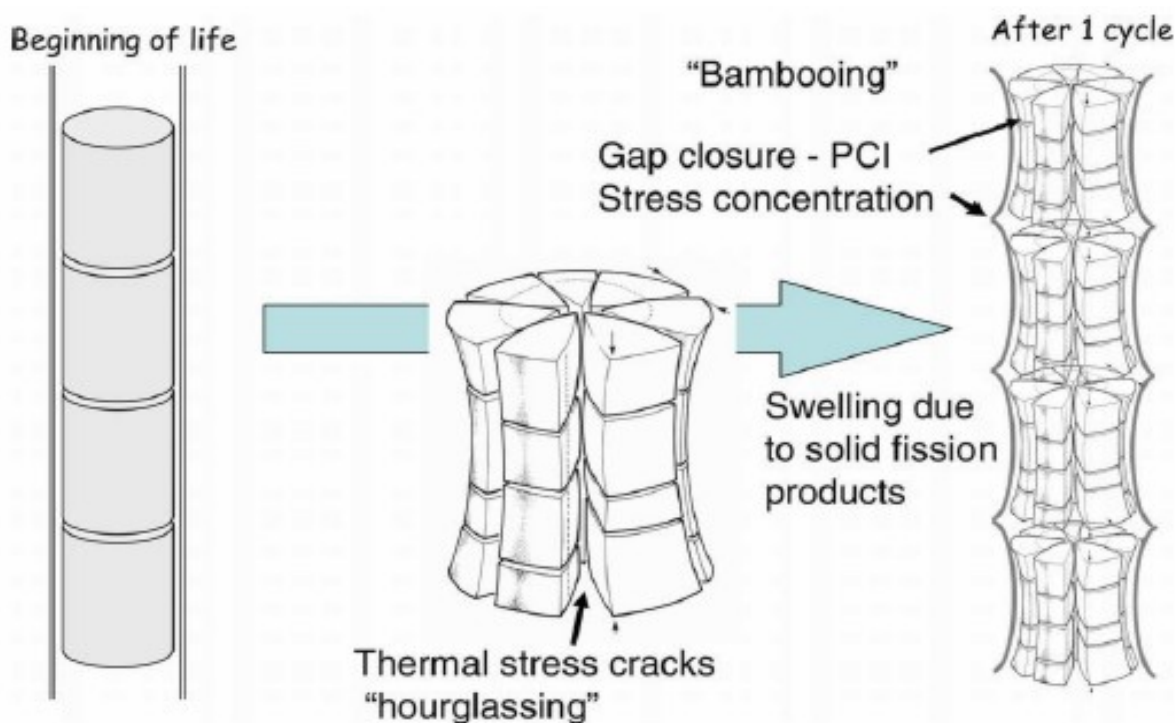
Figure 14. Effects of Fuel-Pellet Swelling and Thermal Stresses 46 (Note: PCI stands for pellet-cladding interaction)
