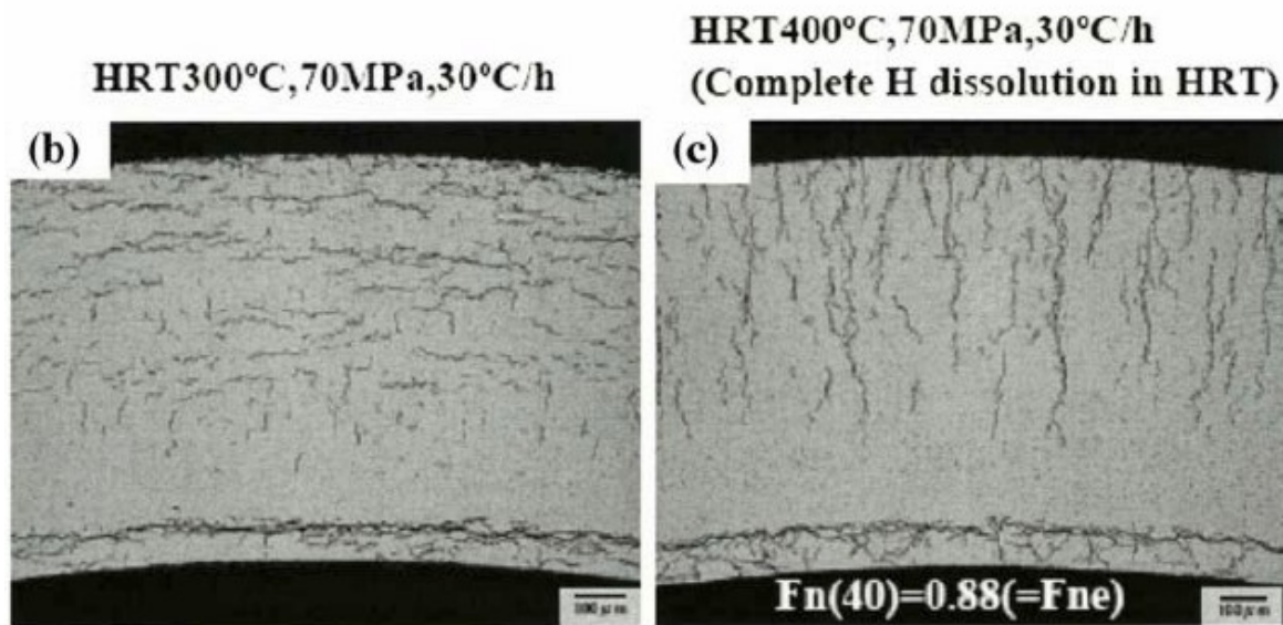
Figure 35. Large Radial Hydrides in High-Burnup Fuel-Rod Cladding After Cooling 137
