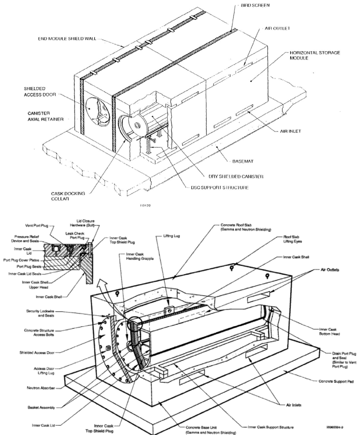
Figure 12. Horizontal Concrete-Shielded Dry-Storage System Used with permission of Transnuclear
