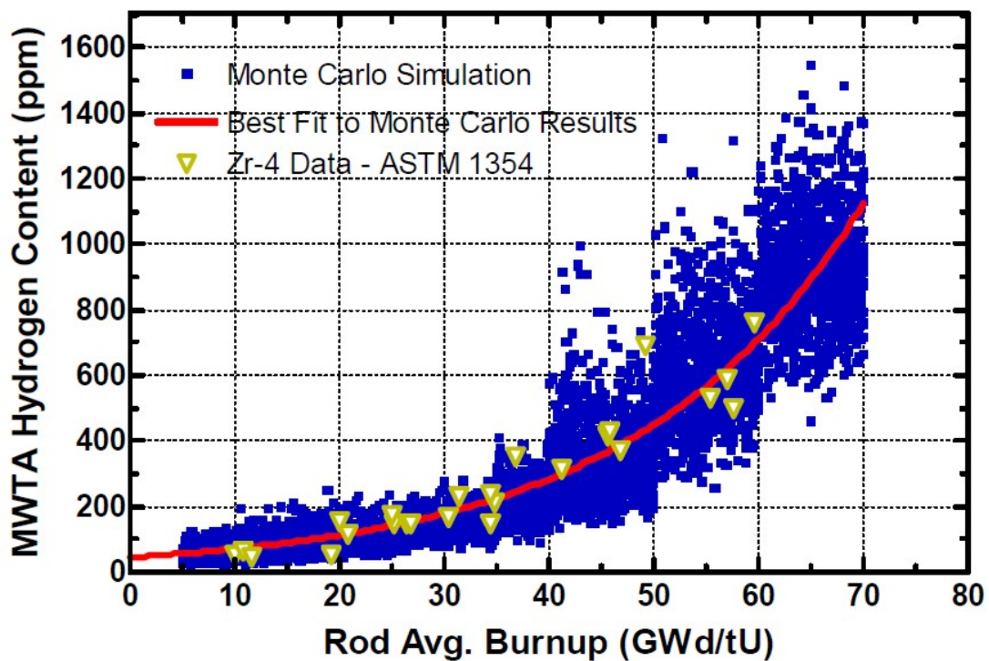
Figure 21. Maximum Wall Thickness Average (MWT) Hydrogen Content in Low-Tin Zircaloy-4 Cladding 63
