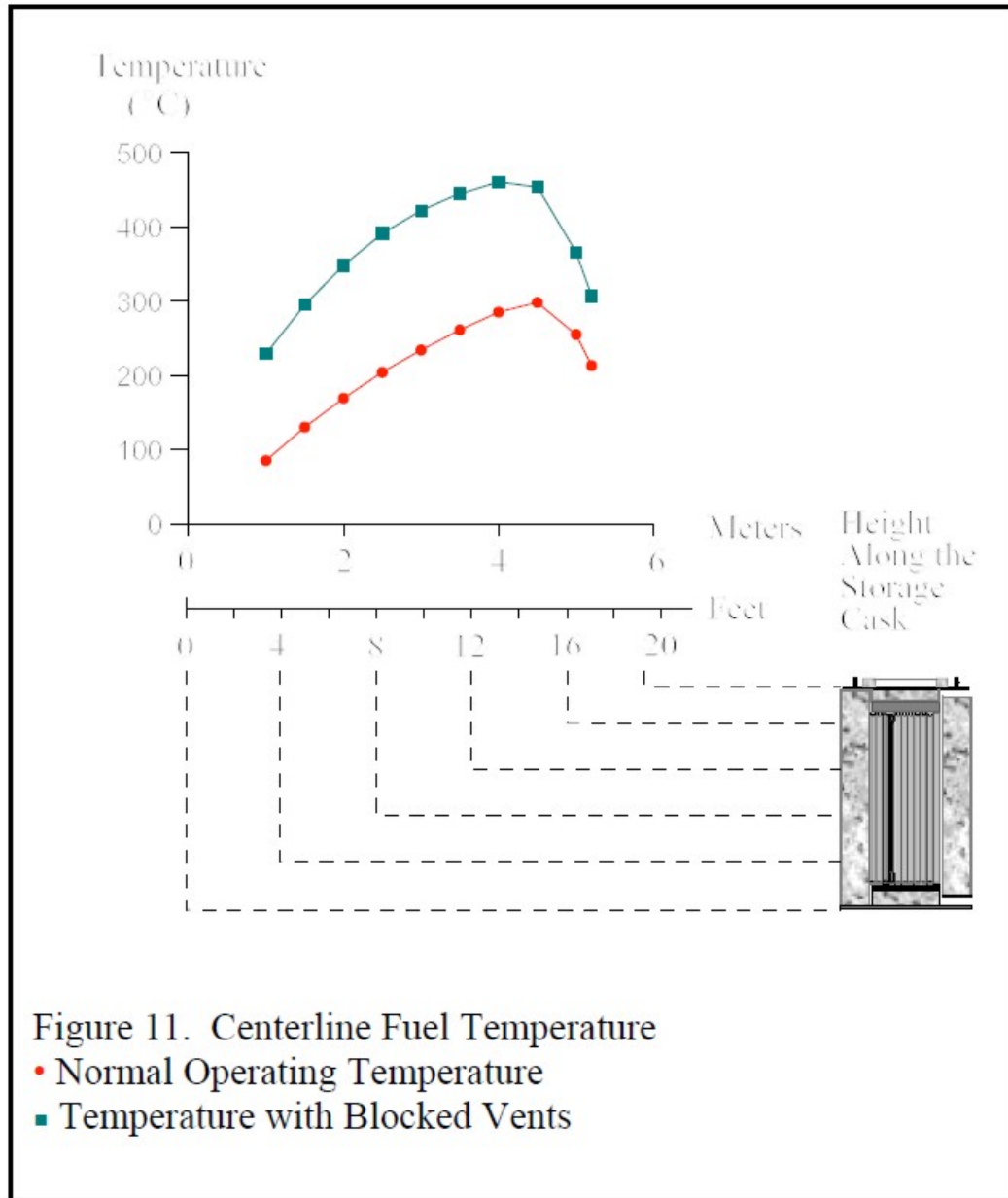
Figure 31. MPC Centerline Fuel Temperature as a Function of Height (unknown fuel age, best available figure) 84
